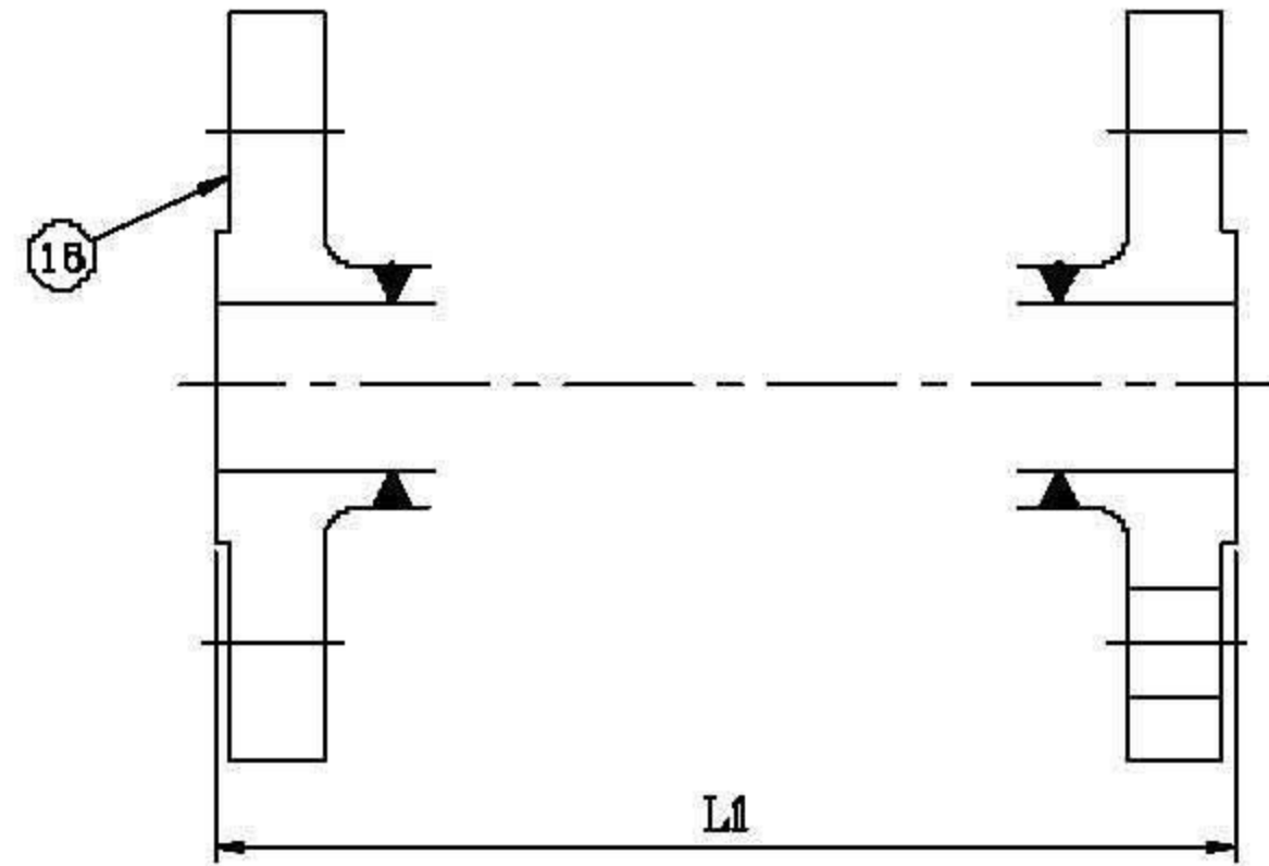
Flanged Ends
